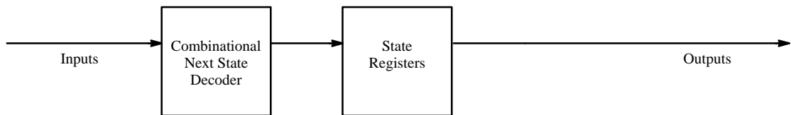
Class C (registered output Moore) FSM
