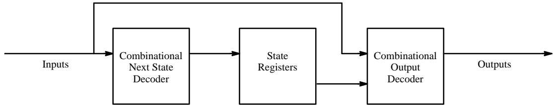
Class A (combinational output Mealy) FSM
