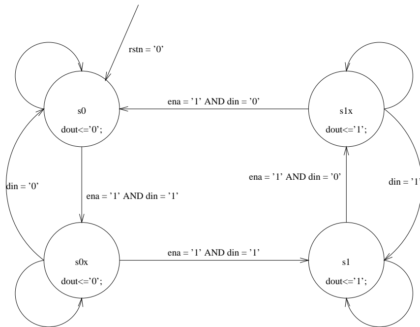
Figure 2. Moore Bounce Suppression Example
